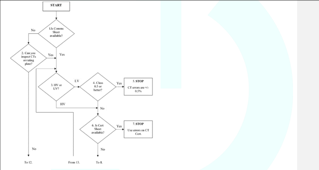
Flowchart for CTs (use similar process for VTs)
